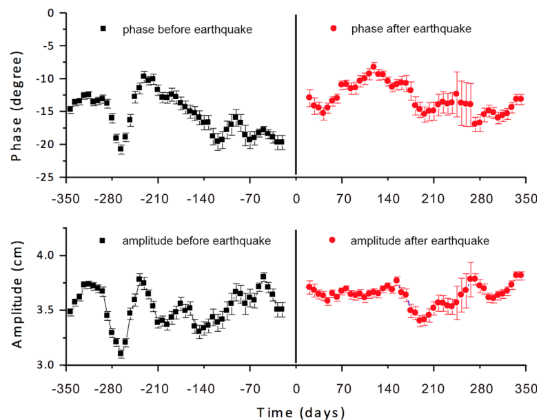
Figure 6. Amplitude and phase shift for water-level response to the M2 tide in Well 3 at Potze Station plotted against time 1 year before and 1 year after the Chi-Chi earthquake (window length of 30 days, overlap of 23 days). Each point represents the amplitude or the phase shift calculated for a data window. Time of the earthquake is marked by a vertical line at t = 0 .
