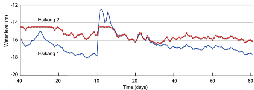
Figure 3. Daily average of water levels in two wells at the Hsikang Station (see Figure 1 for location) before and after the Chi-Chi earthquake, recorded by piezometers located at depths of 40 m (Hsikang 1) and 99 m (Hsikang 2), respectively. Water level is referenced to the mean sea level, with positive values above sea level and negative values below sea level. Time of the earthquake is marked by a vertical line at t = 0 . Positive numbers are days after the earthquake and negative numbers are days before the earthquake. The wells are open to aquifers separated by an aquitard ~40 m thick (see Figure 2b for lithology and screen depths).
