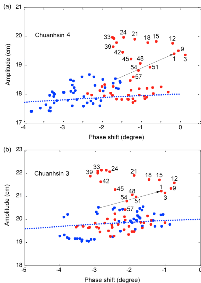
Figure 10. Amplitude versus phase shift for water-level response to the M2 tide in two wells at the Chuanshsin Station. In each well, each point represents the phase shift and amplitude calculated for a data window. Before the earthquake, data points in both wells (blue dots) fit a confined aquifer model (dashed line) [Hsieh et al., 1987]. Coseismic changes in both wells are given by arrows that connect the last pre-seismic data point to the first postseismic data point. Data points during the first ~60 days after the earthquake are numbered in sequence to show the time-dependent evolution. Both the arrows and the postseismic data points during the first ~60 days after the earthquake deviate significantly from the trend defining a confined aquifer (dashed line), which we refer in the text as the “excursion” from a confined aquifer. Numbering refers to the number of days after the earthquake and the first day in a data window.
